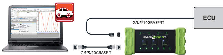
Using the RAD-Moon 3 as a media converter.
